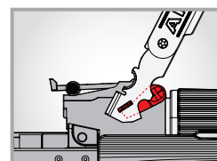
Disassemble gas tube
